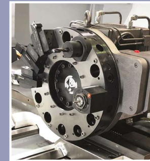
Turret for driven tools with options for C-axis spindle positioning: - driven by main motor - in combination with hydraulic brake and spindle encoder - full contouring C-axis driven directly by separate servo motor
